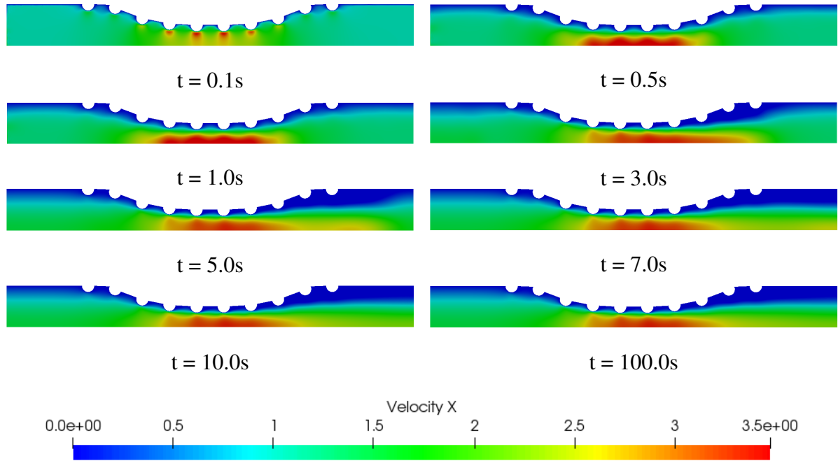
Figure 44: Temporal and spatial evolution of the velocity field for quadratic curved channel with drug-eluting stent.
