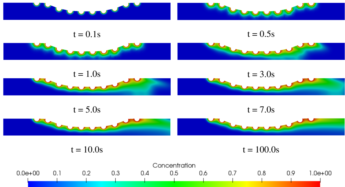
Figure 45: Temporal and spatial evolution of the concentration field for quadratic curved channel with drug-eluting stent and Sc = 1 .
