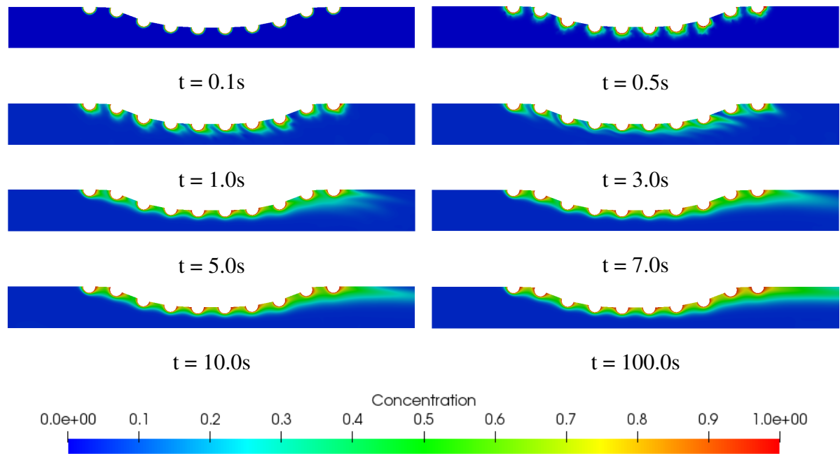
Figure 46: Temporal and spatial evolution of the concentration field for quad curved channel with drug-eluting stent and Sc = 10 .
